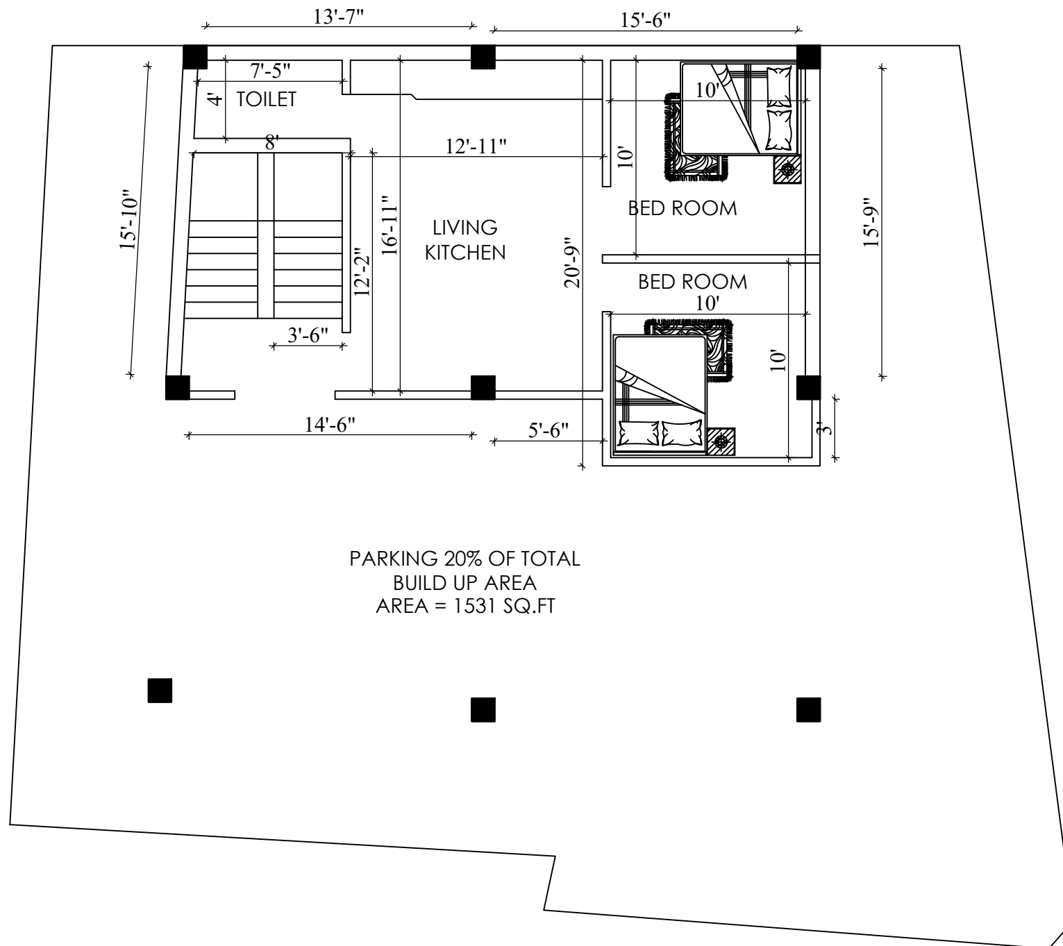
GROUND FLOOR PLAN AREA = 1190 SQ.FT
